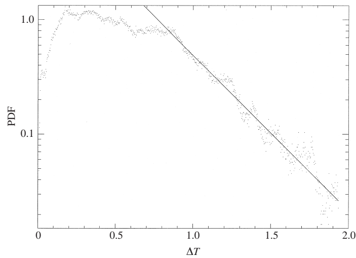
FIGURE 14. PDF of the temperature fluctuation ( \delta T = T - T_0 ) within the mixing zone ( \Delta z = 0.025 ) at z = 0.21 .
